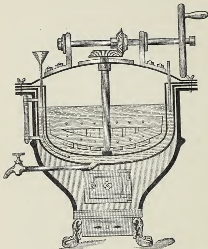
FIG. 24.—Zemsch's Spirit-varnish Apparatus.
